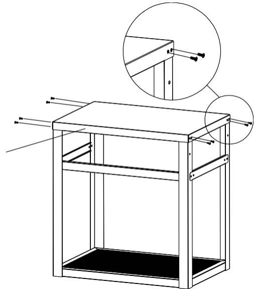
2. A M6*15 6PCS
